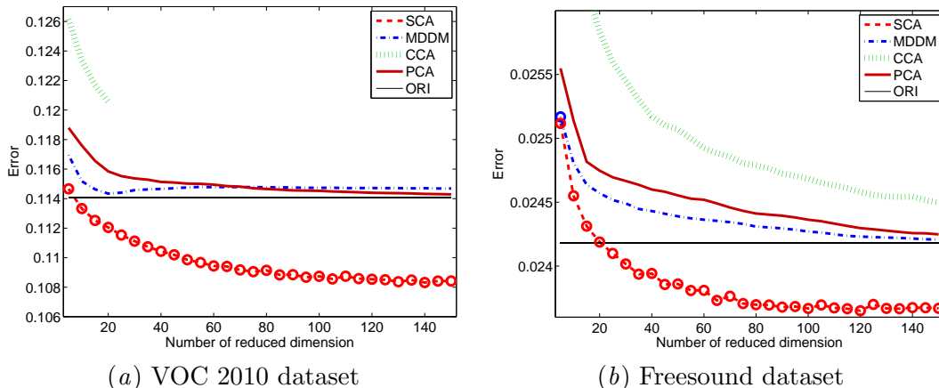
Figure 2: Results on image classification with VOC 2010 dataset and audio classification with Freesound datasets. Misclassification rates when the one-nearest-neighbor classifier is used as a classifier are reported. The best dimension reduction method achieving the smallest mean error and comparable methods according to the t-test at the significance level 1% are specified by ‘o’. CCA can be applied to dimension reduction up to c dimensions, where c is the number of classes ( c = 20 in VOC 2010 and c = 230 in Freesound). ‘ORI’ denotes the original data without dimension reduction.
